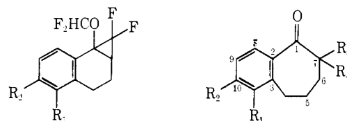
8a , R_1 = \text{OMe}; R_2 = \text{H} b , R_1 = \text{H}; R_2 = \text{OMe} 9a , R_2 = \text{OMe}; R_2 = \text{H}; R_3 = R_4 = \text{F} b , R_1 = \text{H}; R_2 = \text{OMe}; R_3 = R_4 = \text{F} c , R_2 = \text{OMe}; R_1 = R_3 = \text{H}; R_4 = \text{F} d , R_2 = \text{OMe}; R_1 = R_3 = R_4 = \text{H}
