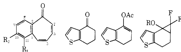
10a , R_1 = \text{OMe}; R_2 = \text{H} b , R_1 = \text{H}; R_2 = \text{OMe} 11 12 13a , R = \text{Ac} b , R = \text{CHF}_2
